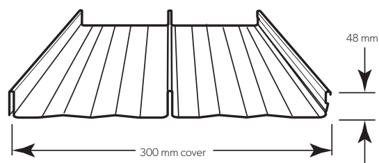
Fluted LONGLINE 305®
