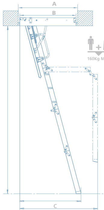
4 SEGMENT LADDERS
